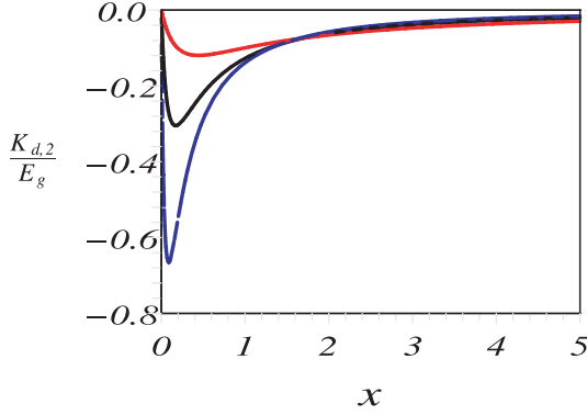
Fig. 1. K_{d,2}/E_g versus x = \gamma/\mathbf{w}_0 , where the ground state energy E_g = \frac{\hbar}{2} \sqrt{\Omega\gamma + \mathbf{w}_0^2} ; for \Omega = 2\mathbf{w}_0 (dot), 5\mathbf{w}_0 (solid), 10\mathbf{w}_0 (dashed) from top to bottom.
